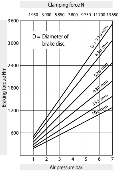
Brake Caliper DV 035 PFM - 655
